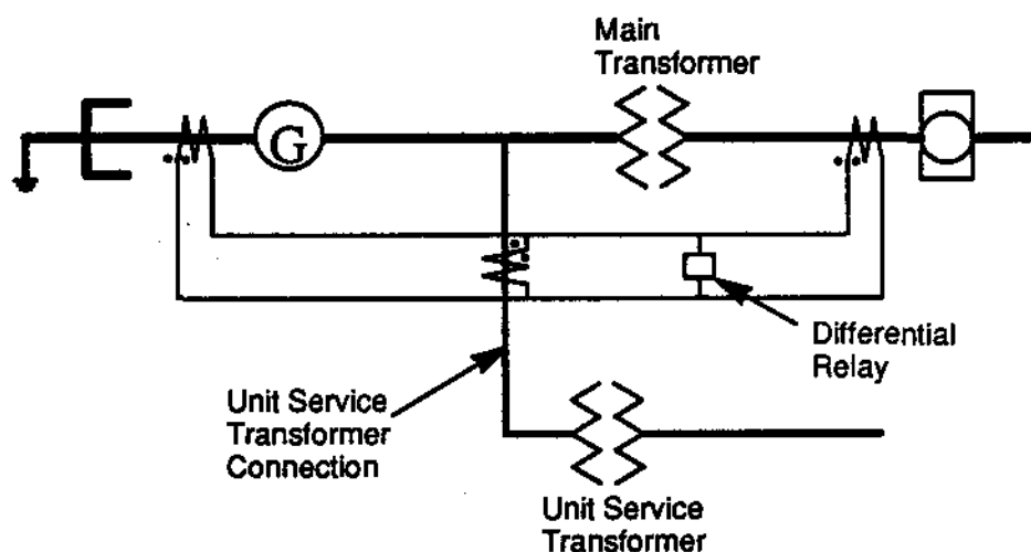
Figure 7.2: Differential Protection Scheme For The Generator (and Main Transformer)
